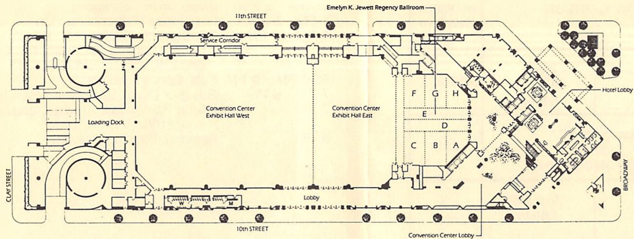
Lower Floor
